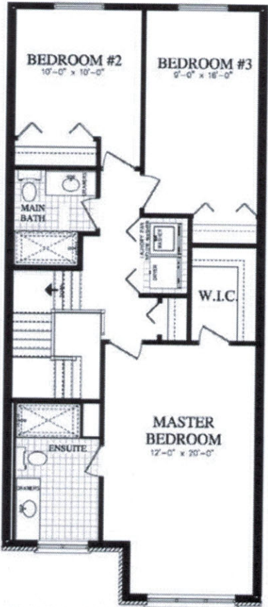
STANDARD GEORGIAN BAY SECOND FLOOR PLAN AREA: 910.0 sq.ft.
